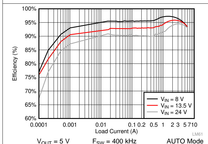
Figure 39. LM61460-Q1 Efficiency
