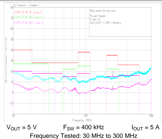
Figure 80. Radiated EMI Bicon Horizontal versus CISPR25 Limits
