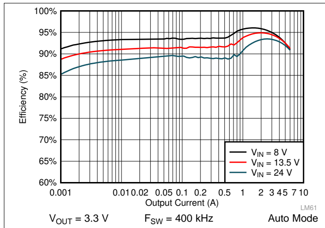
Figure 35. LM61460-Q1 Efficiency
