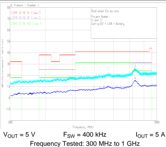
Figure 81. Radiated EMI Log Vertical versus CISPR25 Limits
