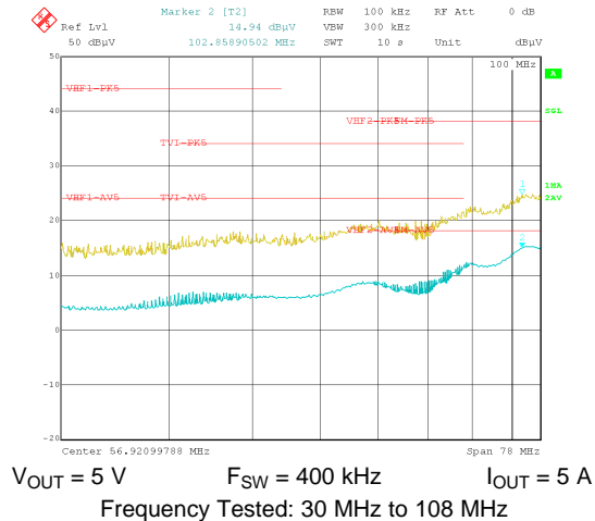
Figure 77. Conducted EMI versus CISPR25 Limits (Yellow: Peak Signal, Blue: Average Signal)
