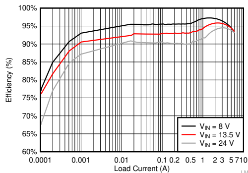
Efficiency: V_{OUT} = 5\text{ V} , F_{SW} = 400\text{ kHz}
