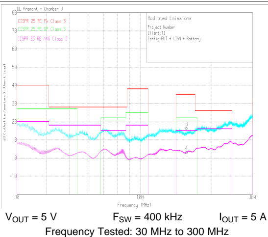
Figure 79. Radiated EMI Bicon Vertical versus CISPR25 Limits
