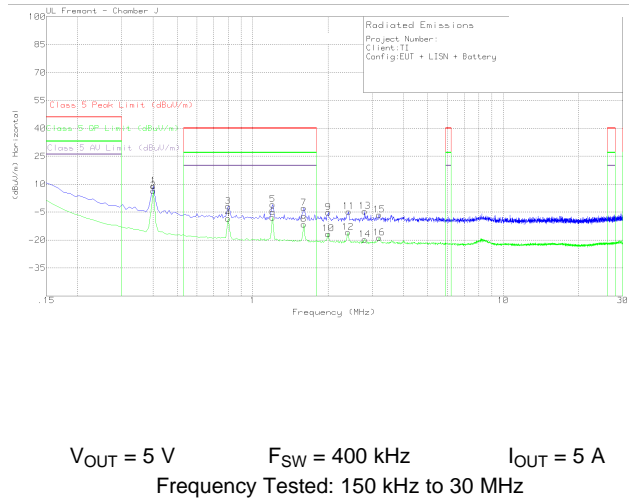
Figure 78. Radiated EMI Rod versus CISPR25 Limits
