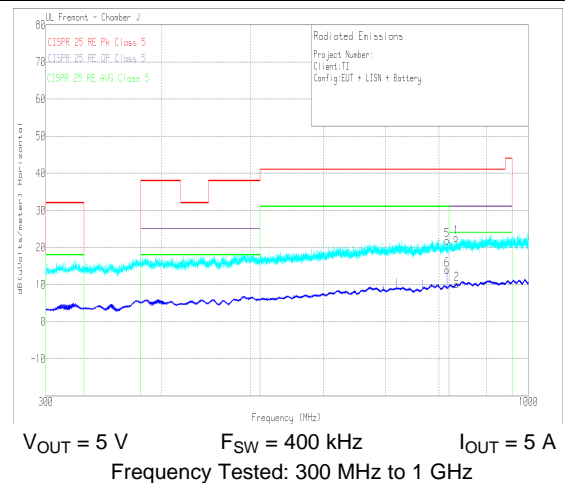
Figure 82. Radiated EMI Log Horizontal versus CISPR25 Limits
