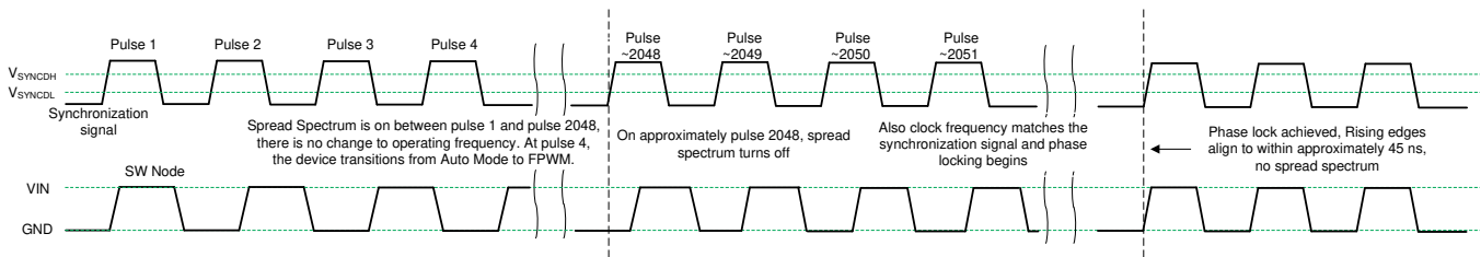
Figure 12. Synchronization Process
