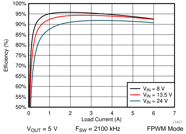
Figure 42. LM61460-Q1 Efficiency
