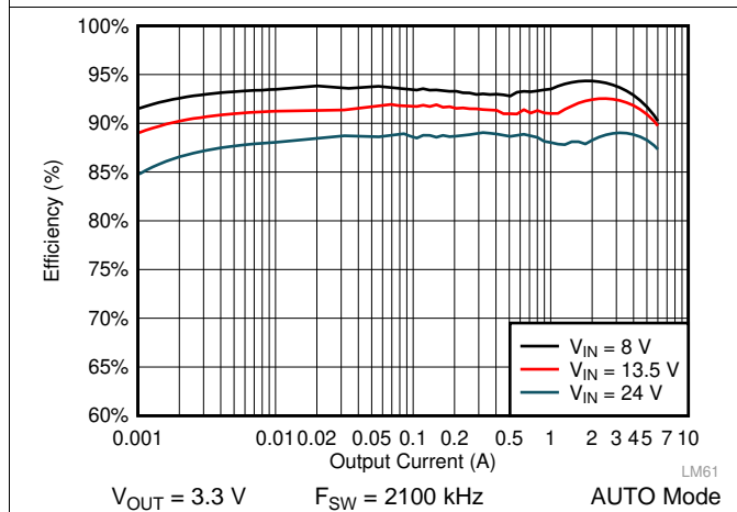
Figure 37. LM61460-Q1 Efficiency
