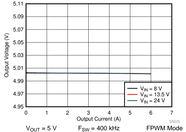
Figure 48. LM61460-Q1 Load and Line Regulation
